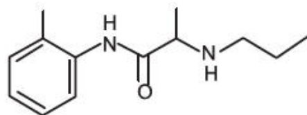
Prilocaine C_{13}H_{20}N_2O M.W. 220.3
