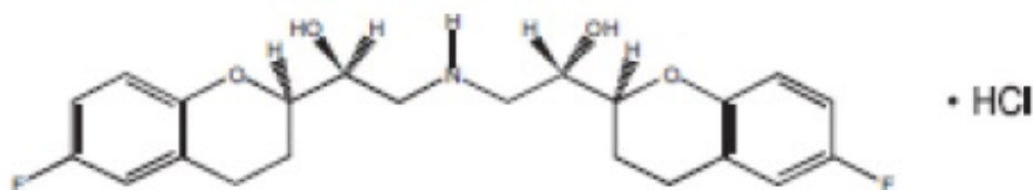
RSSS - or l-nebivolol hydrochloride
