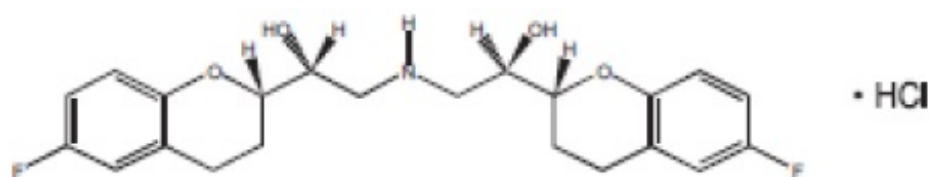
SRRR - or d-nebivolol hydrochloride
