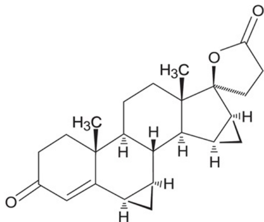
Drospirenone
