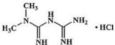
Metformin Hydrochloride
