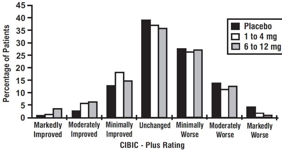
Figure 3: Frequency Distribution of CIBIC-Plus Scores at Week 26 in Study 1
