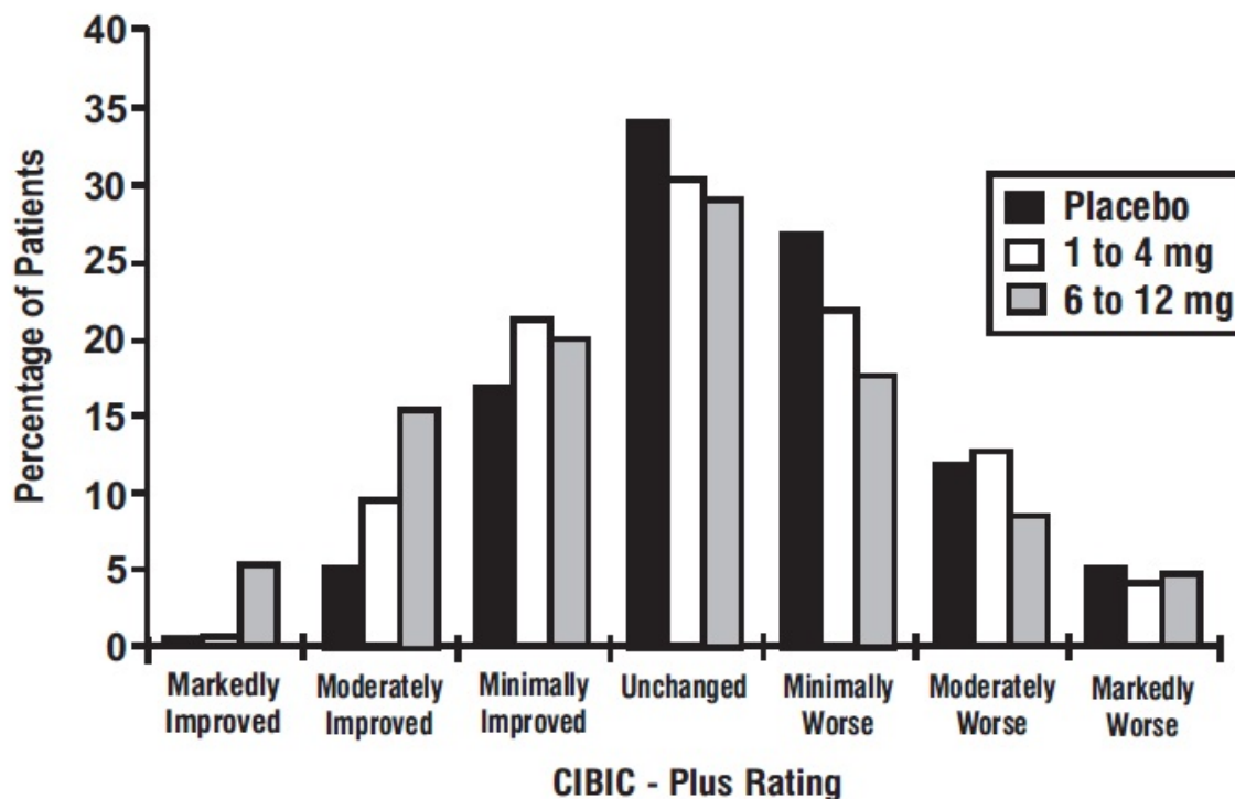
Figure 6: Frequency Distribution of CIBIC-Plus Scores at Week 26 in Study 2
