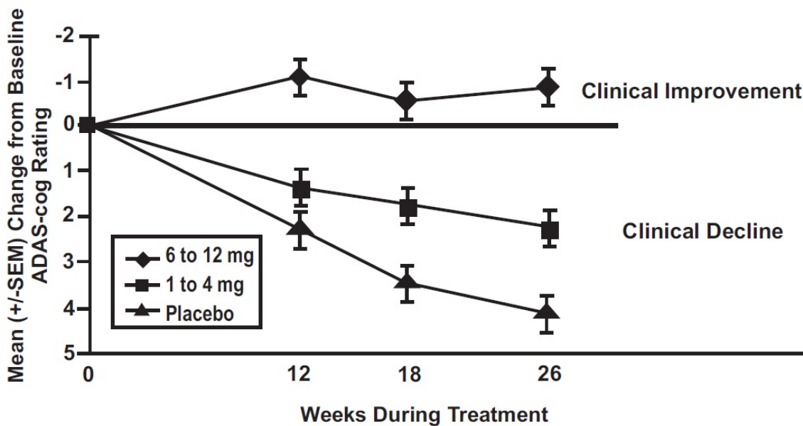
Figure 1: Time-course of the Change from Baseline in ADAS-cog Score for Patients Completing 26 Weeks of Treatment in Study 1
