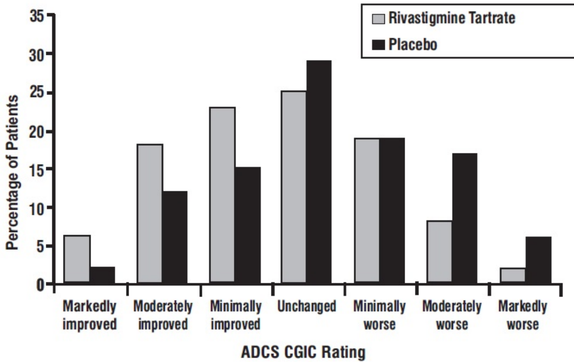
Figure 8: Distribution of ADCS-CGIC Scores for Patients Completing 24 Weeks of Treatment in Study 4
