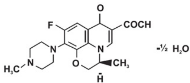
Figure 1: The Chemical Structure of Levofloxacin, USP
