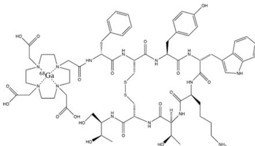
Figure 1: Chemical Structure of Ga 68 DOTATOC
