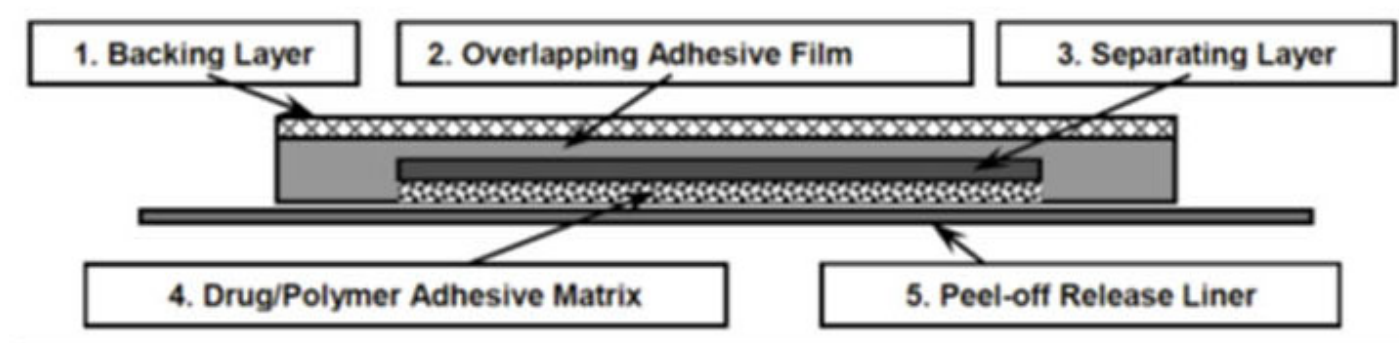
Figure 1: Cross-Section Diagram of Buprenorphine Transdermal System (not to scale).
