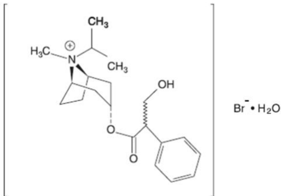
Figure 3.1-2. Chemical structure of ipratropium bromide.
