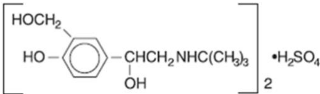
Figure 3.1-1. Chemical structure of albuterol sulfate
