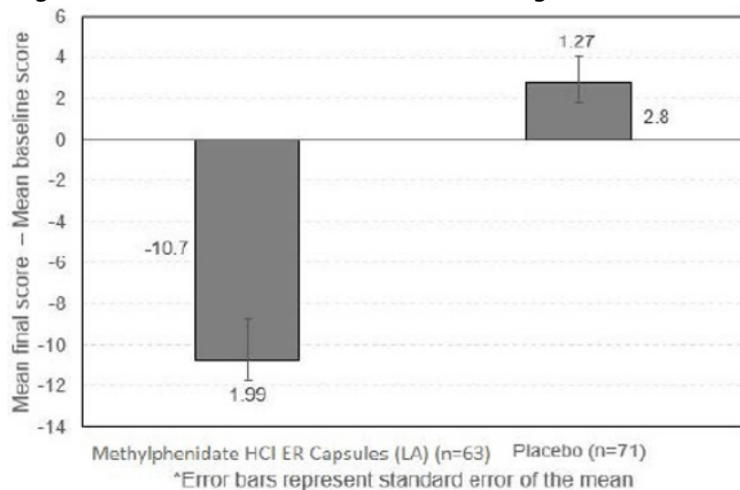
Figure 2: CADS-T Total Subscale - Mean Change From Baseline*
