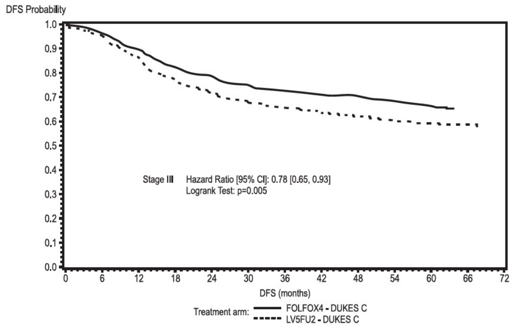
Figure 2: Kaplan-Meier Curves of Disease-Free Survival in Stage III Patients (cutoff: 1 June 2006) in Adjuvant Treatment Trial – ITT Population
