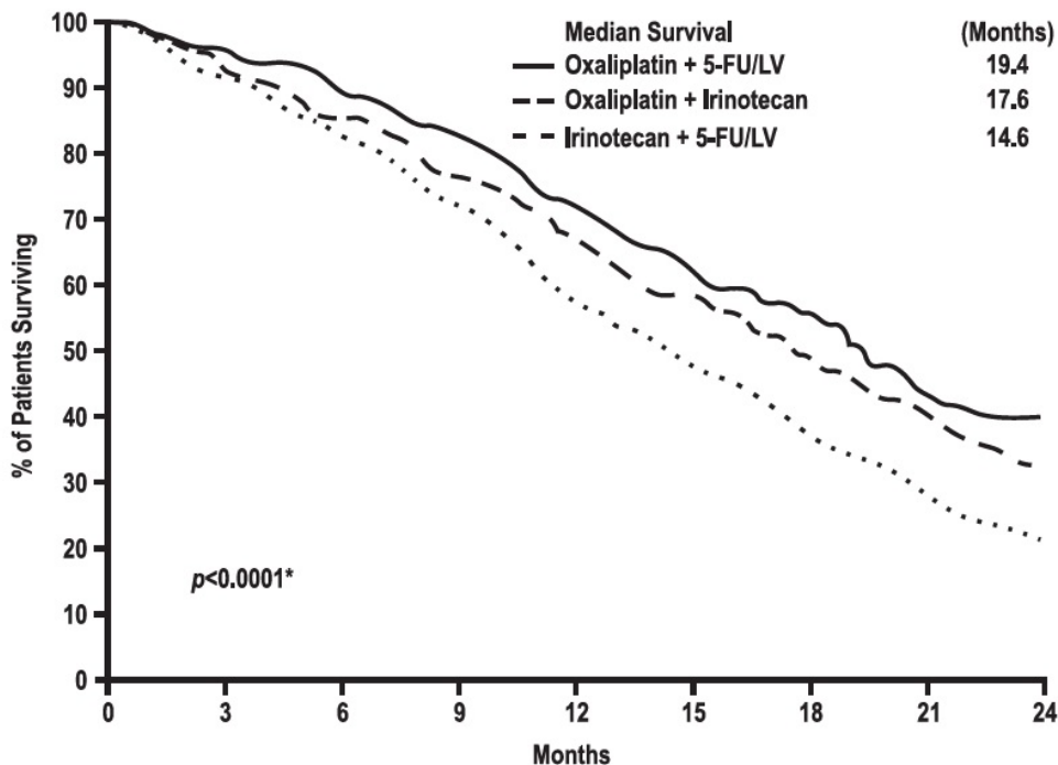
Figure 3: Kaplan-Meier Curves for Overall Survival in Previously Untreated Advanced Colorectal Cancer Trial
