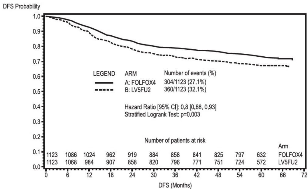
Figure 1: Kaplan-Meier Curves of Disease-Free Survival (cutoff: 1 June 2006) in Adjuvant Treatment Trial – ITT Population
