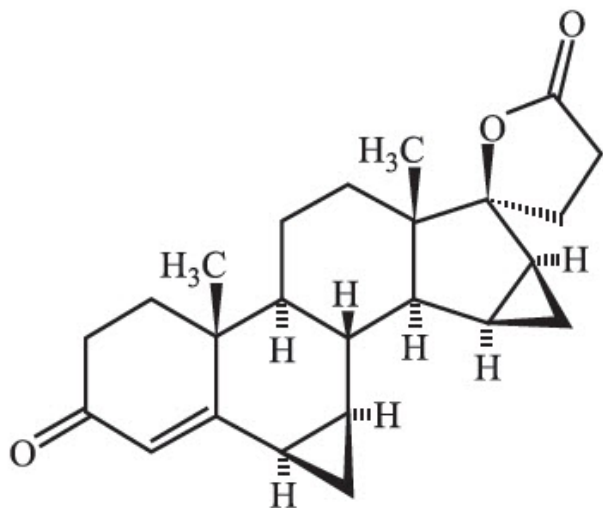
Drospirenone
