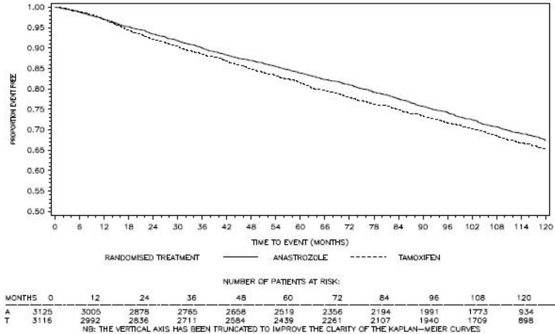
Figure 3 – Disease-Free Survival Kaplan Meier Survival Curve for all Patients Randomized to Anastrozole Tablets or Tamoxifen Monotherapy in the ATAC Trial (Intent-to-Treat) (a)
