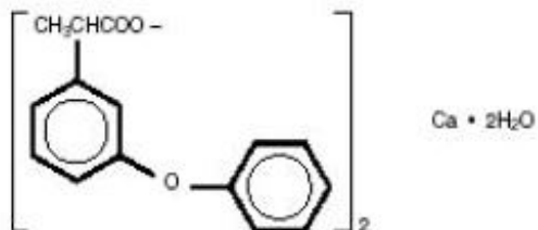
Benzeneacetic acid, \alpha -methyl-3-phenoxy-, calcium salt dihydrate, ( \pm )-
