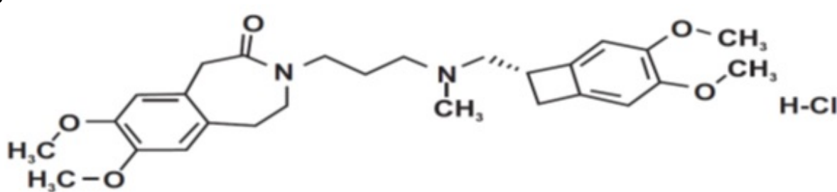
Figure 1. Chemical Structure of Ivabradine
