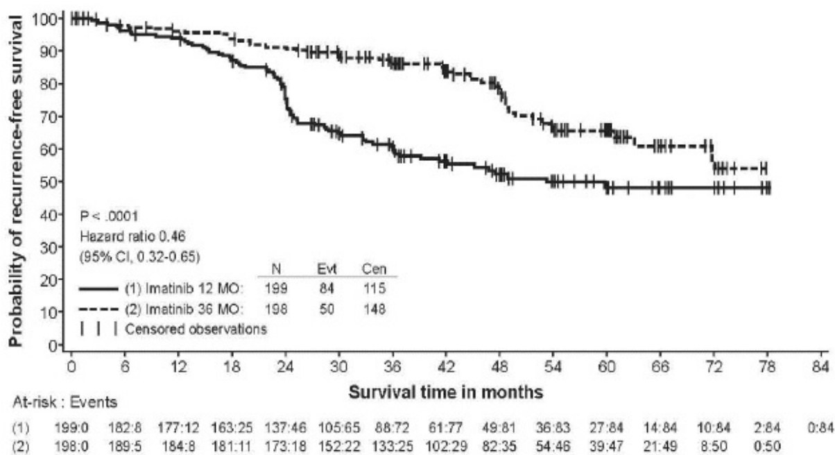
Figure 5: Study 2 Overall Survival (ITT Population)
