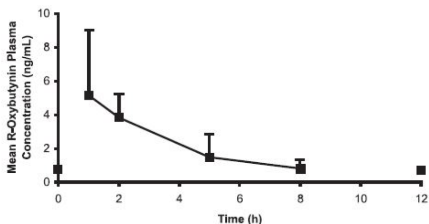
Figure 2. Mean steady-state (±SD) R-oxybutynin plasma concentrations following administration of total daily oxybutynin chloride tablet dose of 7.5 mg to 15 mg (0.22 mg/kg to 0.53 mg/kg) in children 5 to 15 years of age. – Plot represents all available data normalized to the equivalent of oxybutynin chloride 5 mg BID or TID at steady state
