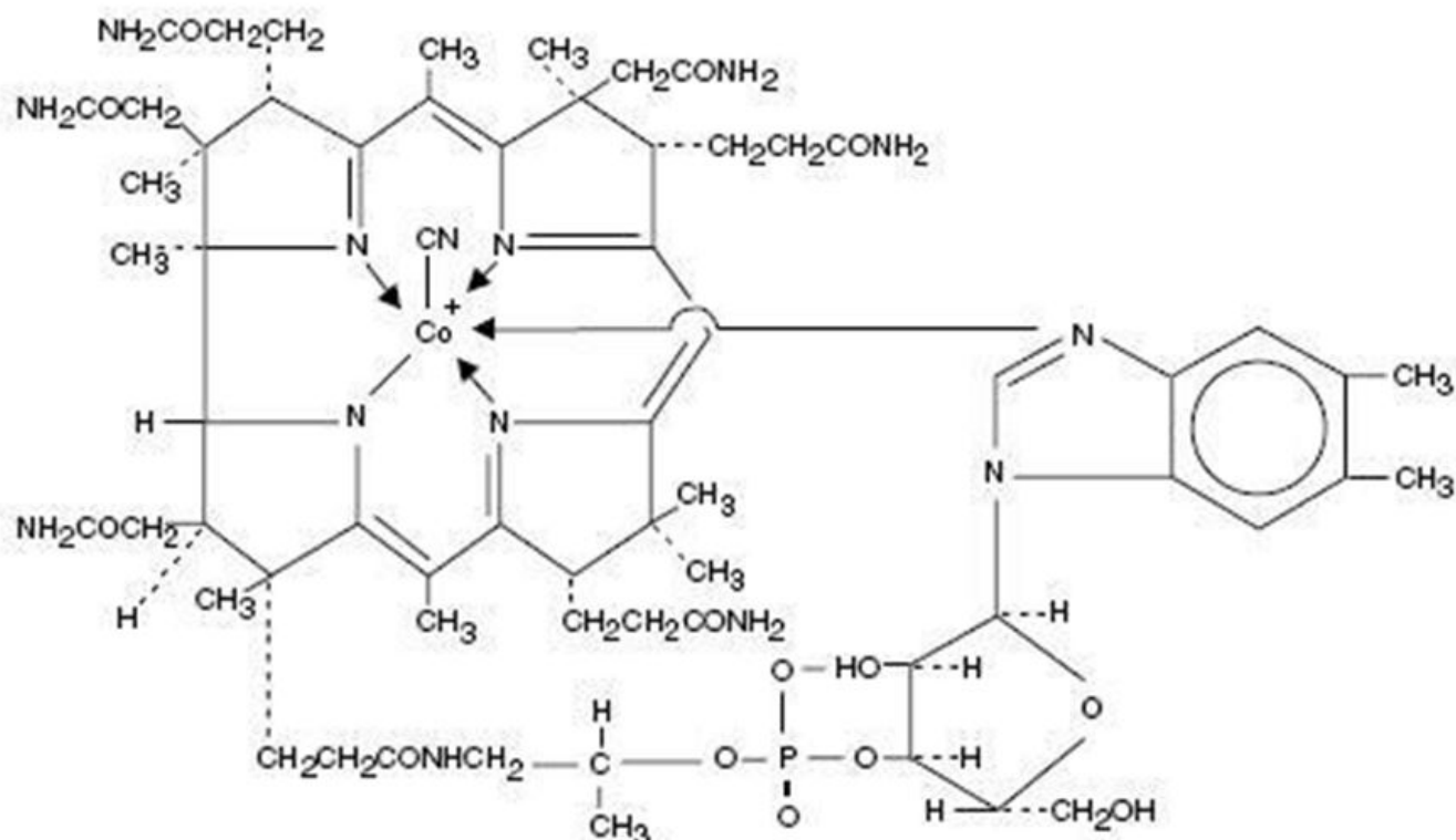
Figure 1. Cyanocobalamin Chemical Structure
