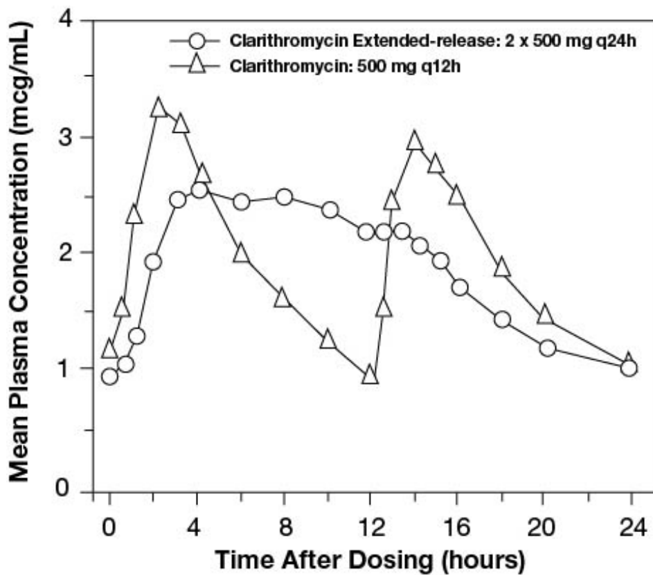
Figure 2: Steady-State Clarithromycin Plasma Concentration-Time Profiles Distribution
