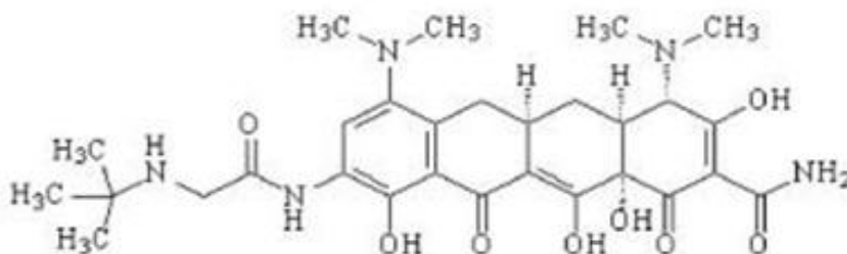
Figure 1: Structure of Tigecycline
