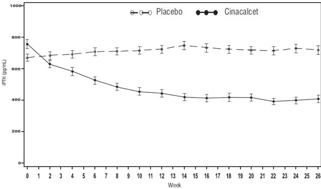
Figure 1. Mean (SE) iPTH Values (Pooled Phase 3 Studies)
