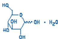
Dextrose Hydrus, USP (β-D-Glucopyranose monohydrate)
