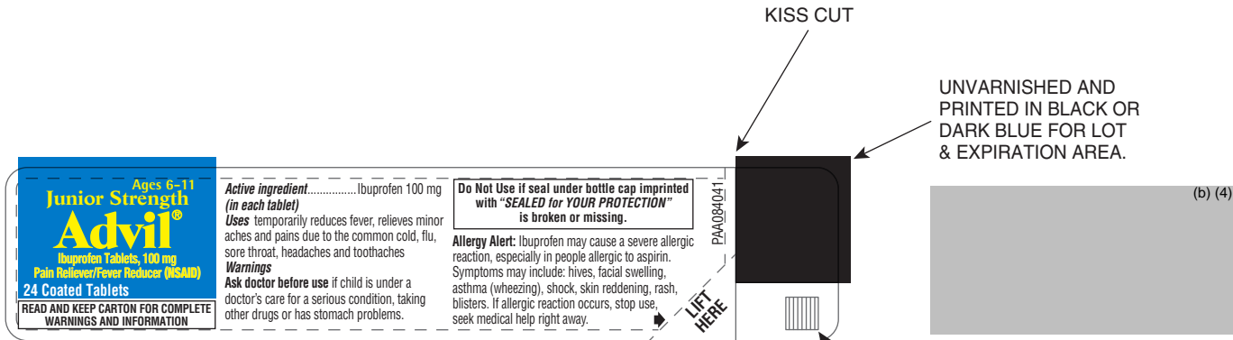
TOP PANEL 1
