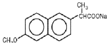
Naproxen sodium Molecular Formula: C 14 H 13 NaO 3 Molecular Weight: 252.24
