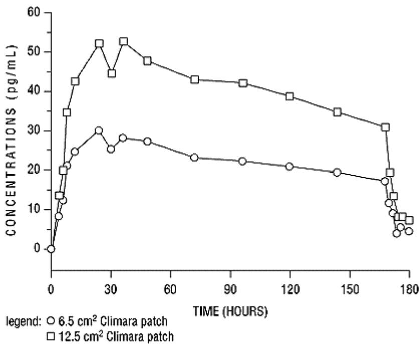
Figure 3 Mean Serum 17β-Estradiol Concentrations vs. Time Profile following Application of a 6.5 cm 2 Transdermal Patch and Application of a 12.5 cm 2 Climara® patch.
