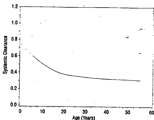
Figure 7: Systemic Clearance (L/hr*kg) of Lamivudine in Relation to Age
