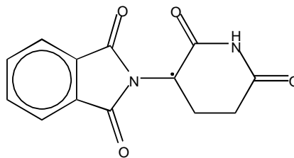
Chemical Structure of Thalidomide
