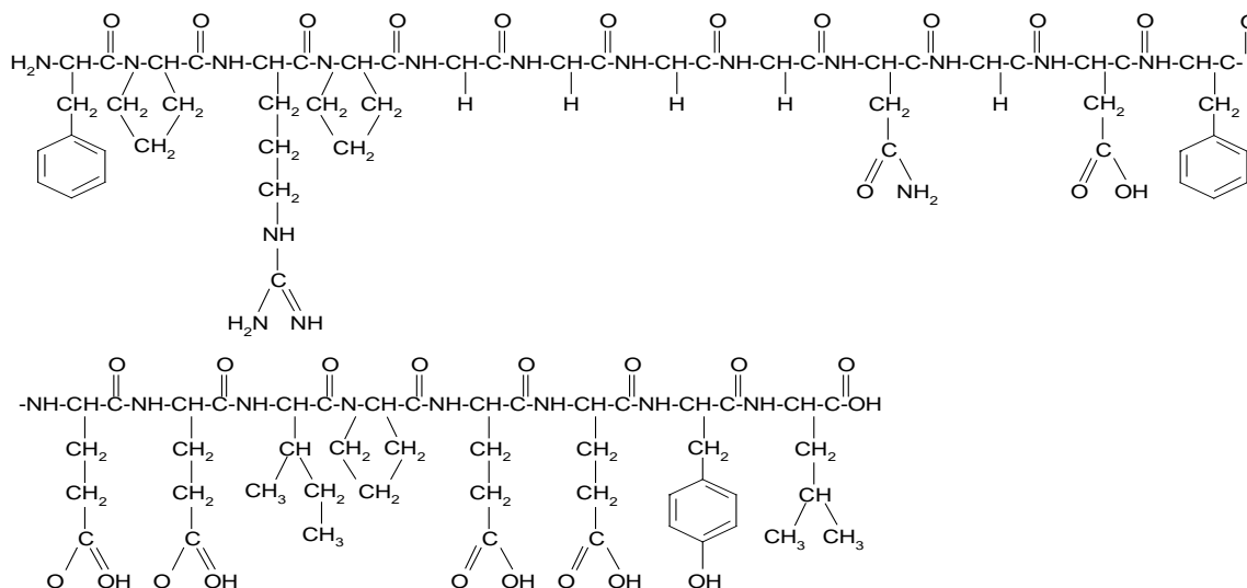
Figure 1. Structural Formula for Bivalirudin
