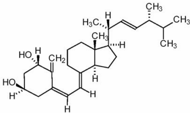
Figure 1: Chemical Structure of Doxercalciferol
