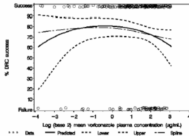
FIGURE 2A Binomial data and logistic fit for DRC therapeutic success versus log plasma concentration --- MITT subjects excluding five subjects with voriconazole plasma concentration > 9mcg/mL
