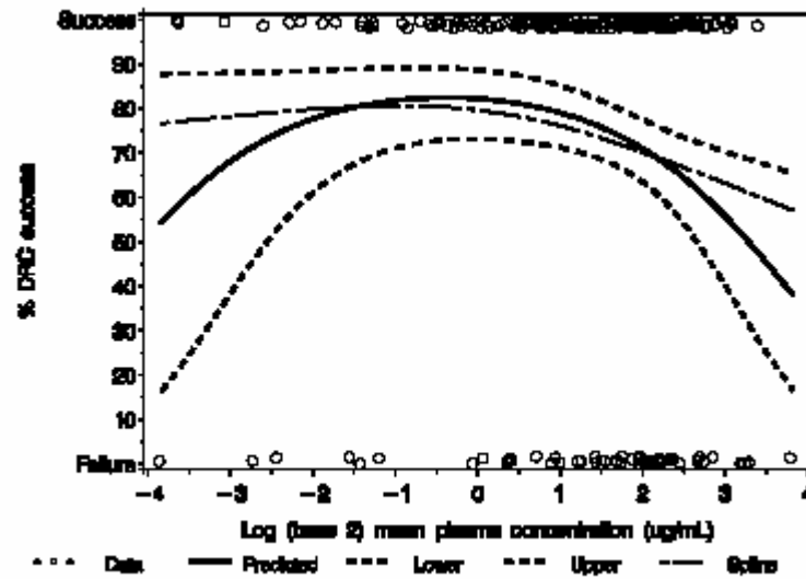
FIGURE 2 Binomial data and logistic fit for DRC therapeutic success versus log plasma concentration --- MITT subjects
