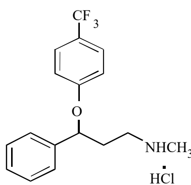
fluoxetine hydrochloride
