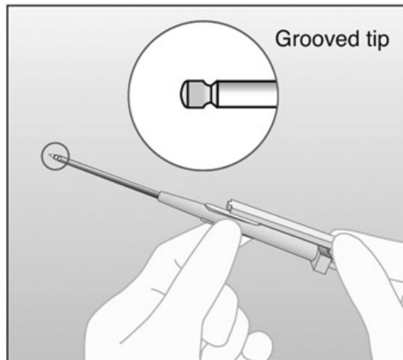
Figure 3b Grooved tip of obturator (enlarged)
