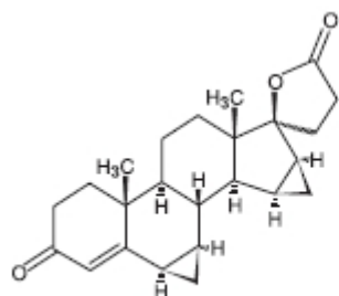
Drospirenone
