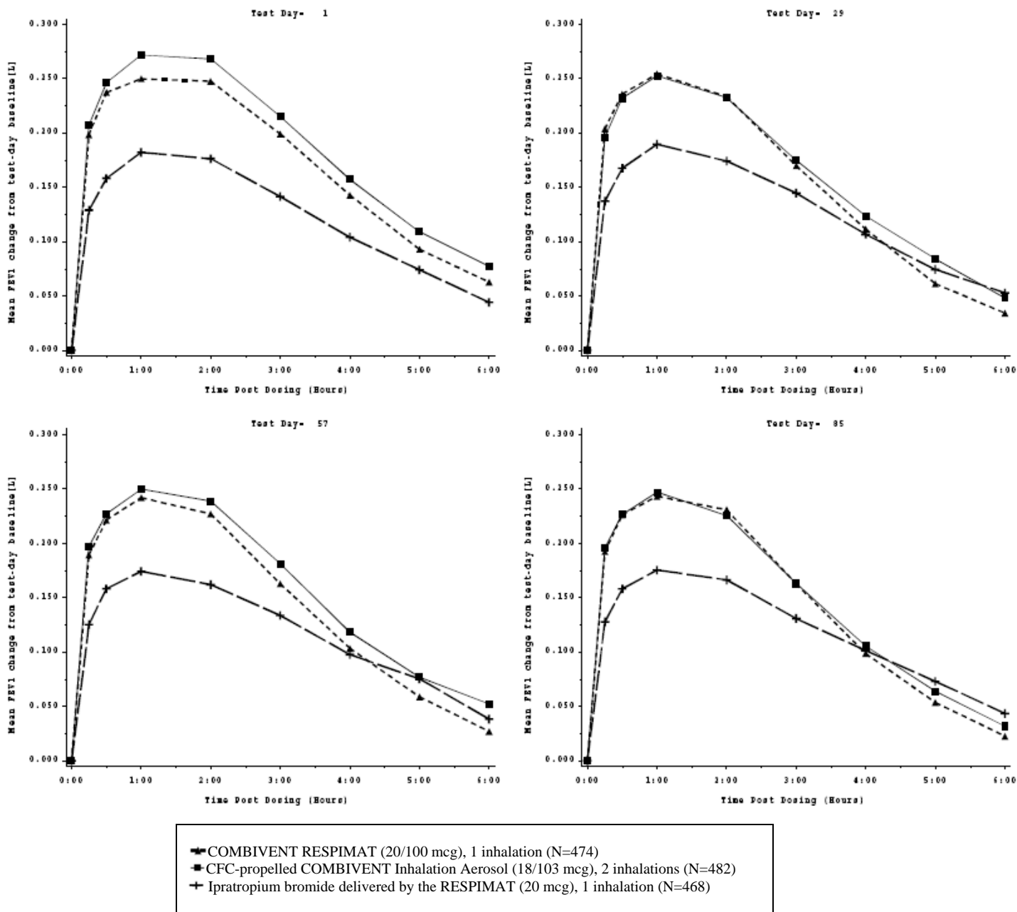
Figure 1 Time Profile of FEV 1 at Days 1, 29, 57, and 85
