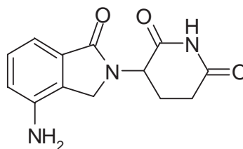
3-(4-amino-1-oxo-1,3-dihydro-2H-isoindol-2-yl) piperidine-2,6-dione
