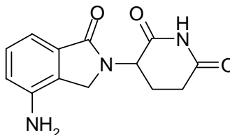
3-(4-amino-1-oxo-1,3-dihydro-2H-isoindol-2-yl) piperidine-2,6-dione
