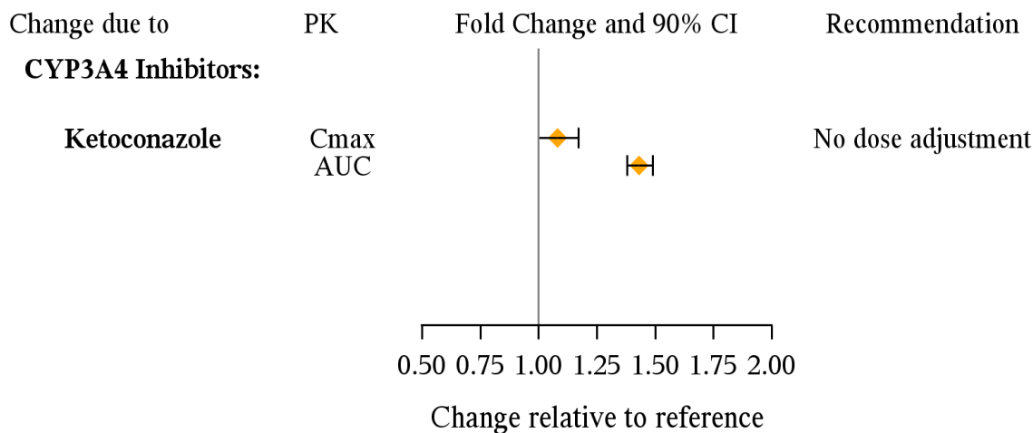
Figure 1. Impact of other drugs on Desvenlafaxine Pharmacokinetics (PK)
