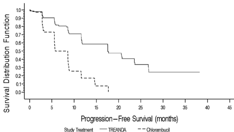
Figure 1. Progression-Free Survival
