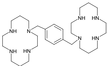
Figure 1: Structural Formula
