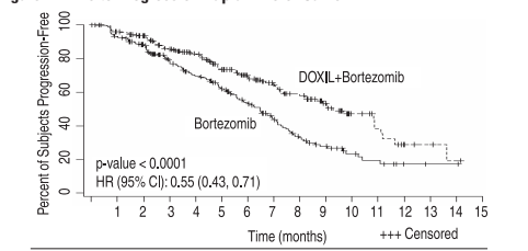
Figure 1- Time to Progression Kaplan-Meier Curve
