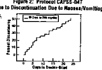
Figure 2: Protocol CAPSS-047
