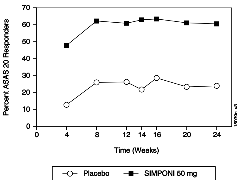
Figure 3: Trial AS – Percentage of AS Patients Achieving ASAS 20 Response by Visit: Randomized Patients *
