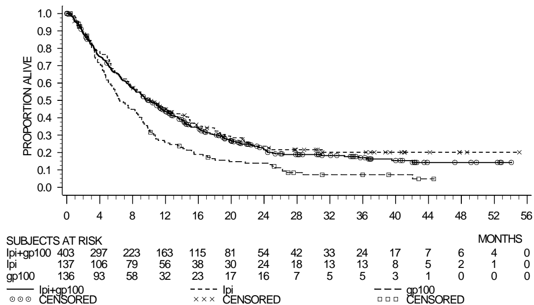
Figure 1: Overall Survival
