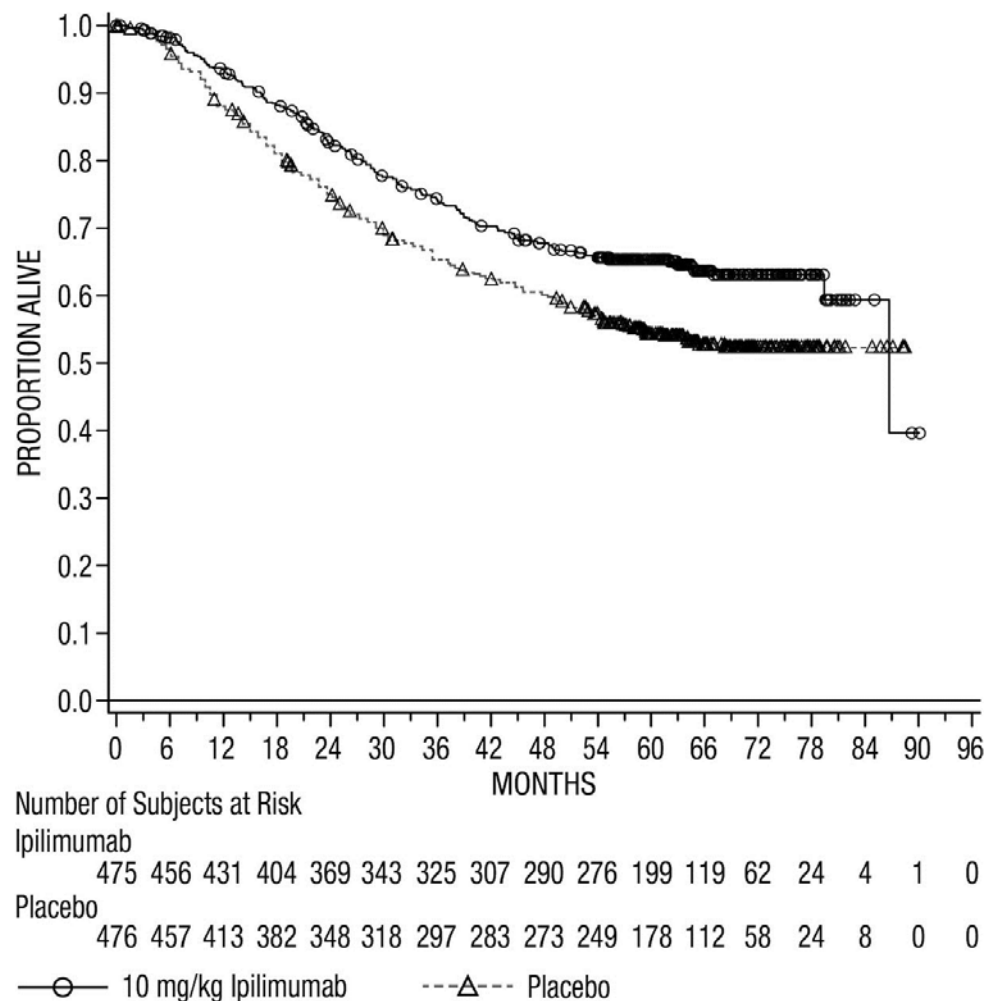
Figure 2: Overall Survival
