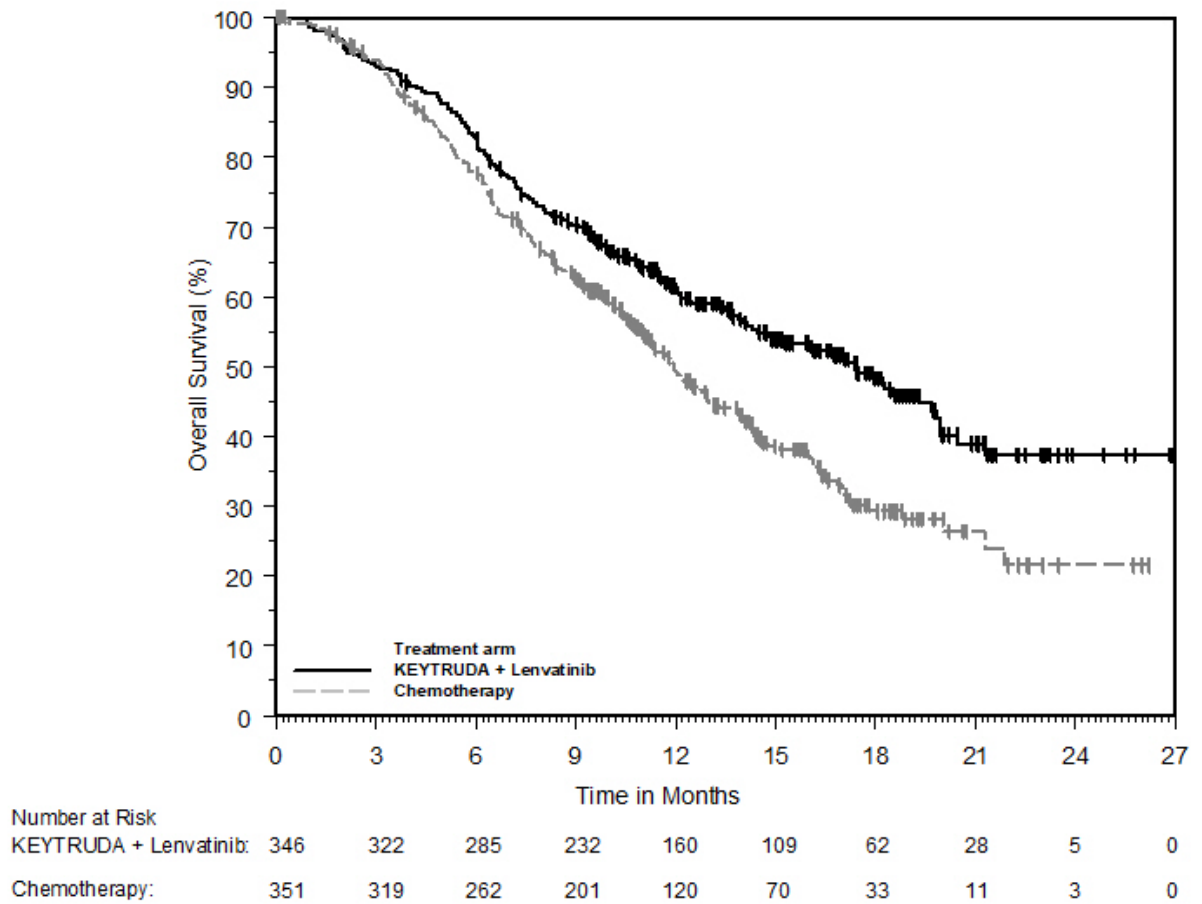
Figure 23: Kaplan-Meier Curve for Overall Survival in KEYNOTE-775 (pMMR or Not MSI-H)
