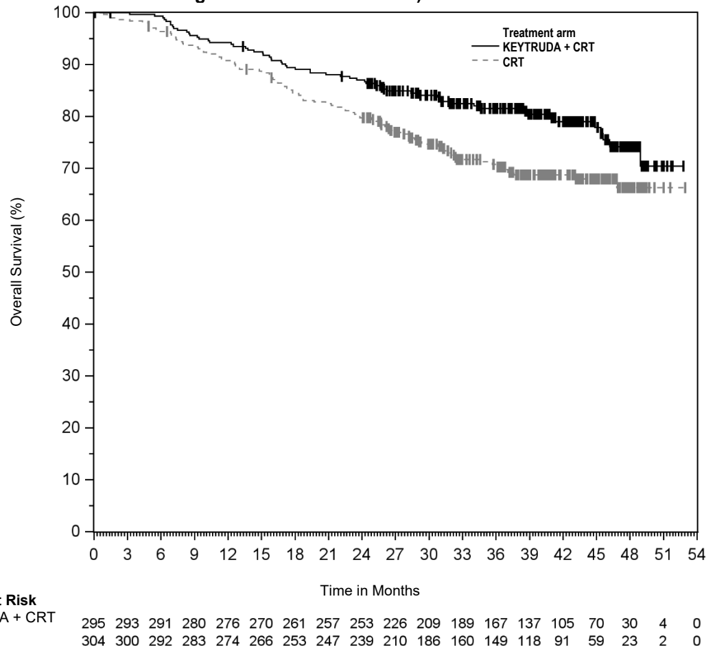
Figure 26: Kaplan-Meier Curve for Overall Survival in KEYNOTE-A18 (Patients with FIGO 2014 Stage III-IVA Cervical Cancer)
