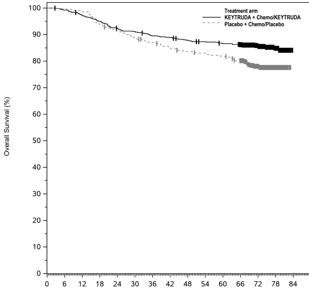
Figure 41: Kaplan-Meier Curve for Overall Survival in KEYNOTE-522
