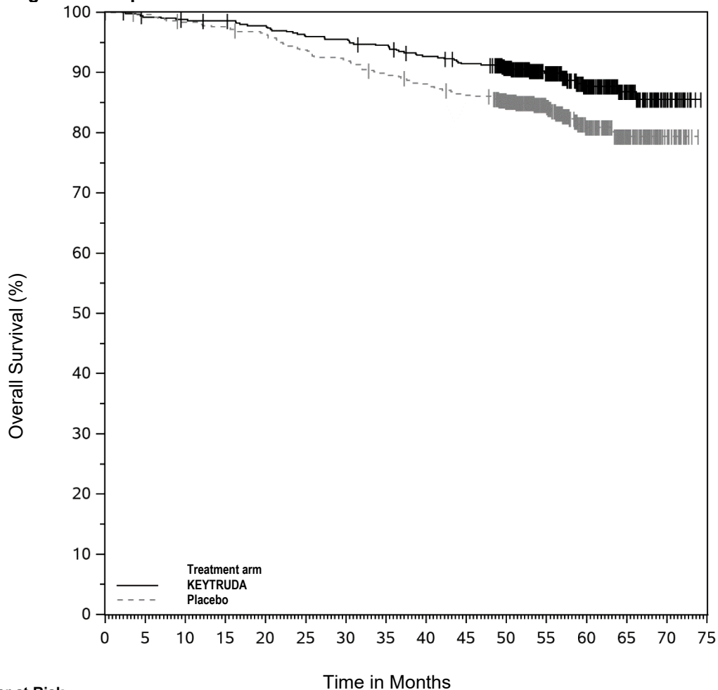
Figure 35: Kaplan-Meier Curve for Overall Survival in KEYNOTE-564
