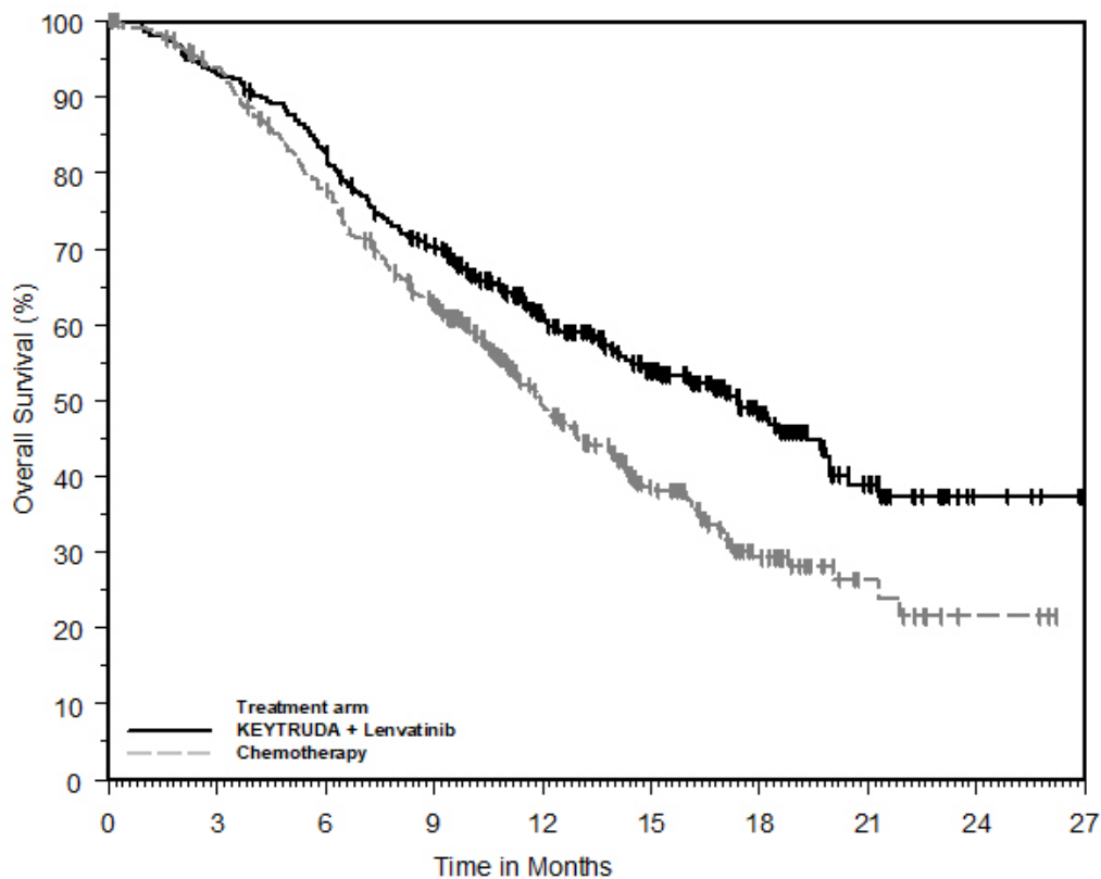
Figure 38: Kaplan-Meier Curve for Overall Survival in KEYNOTE-775 (pMMR or Not MSI-H)
