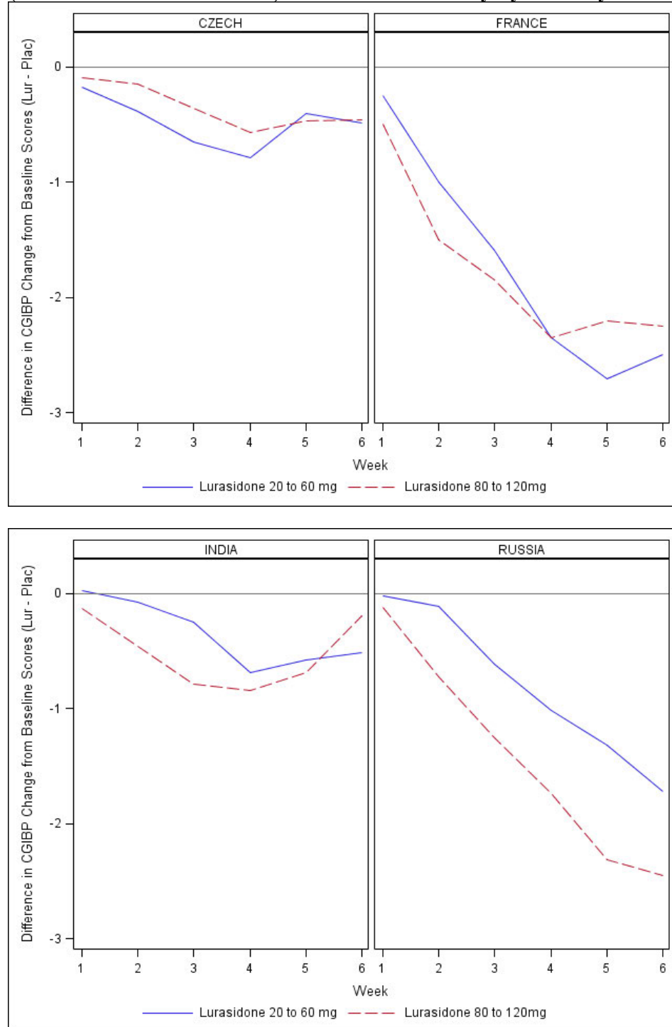
Figure A9: LS Mean Difference in CGI-BP-S Total Score Change from Baseline Scores (Lurasidone minus Placebo) over Course of Study by Country and Dose (MMRM)
