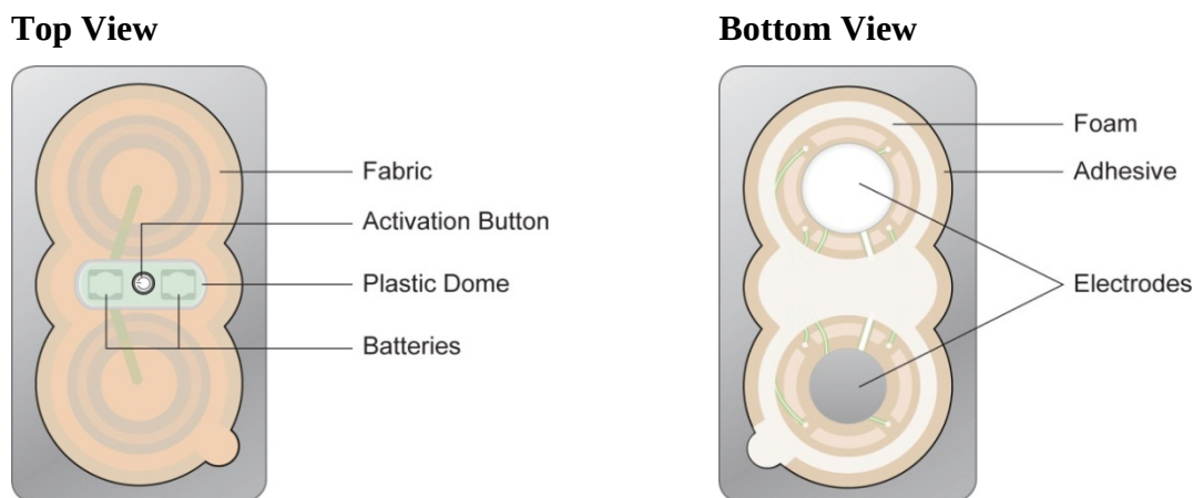
Figure 2: Iontophoretic Device
