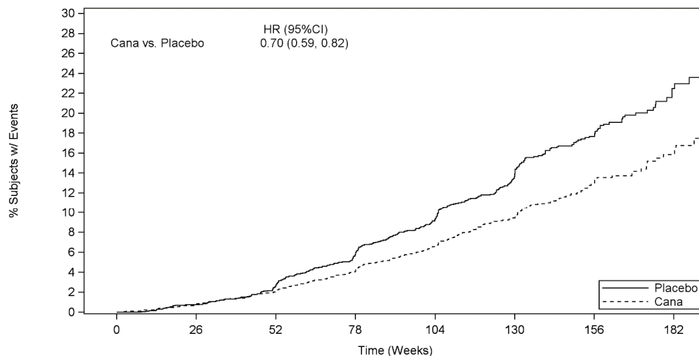
Figure 4: CREDESCENCE: Time to First Occurrence of the Primary Composite Endpoint
