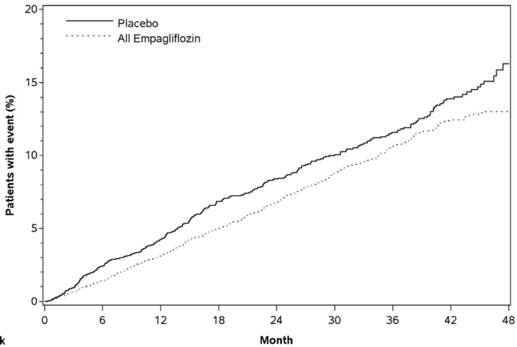
Figure 4 Estimated Cumulative Incidence of First MACE
